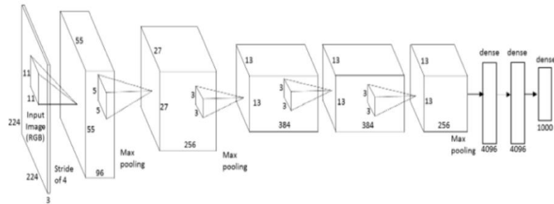
AlexNet
