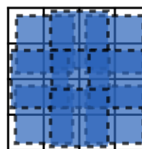
Overlapped Pooling
