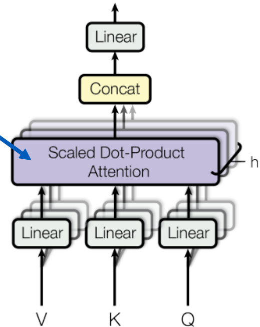
Multi-Head Attention
