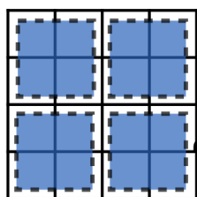
Traditional Pooling
